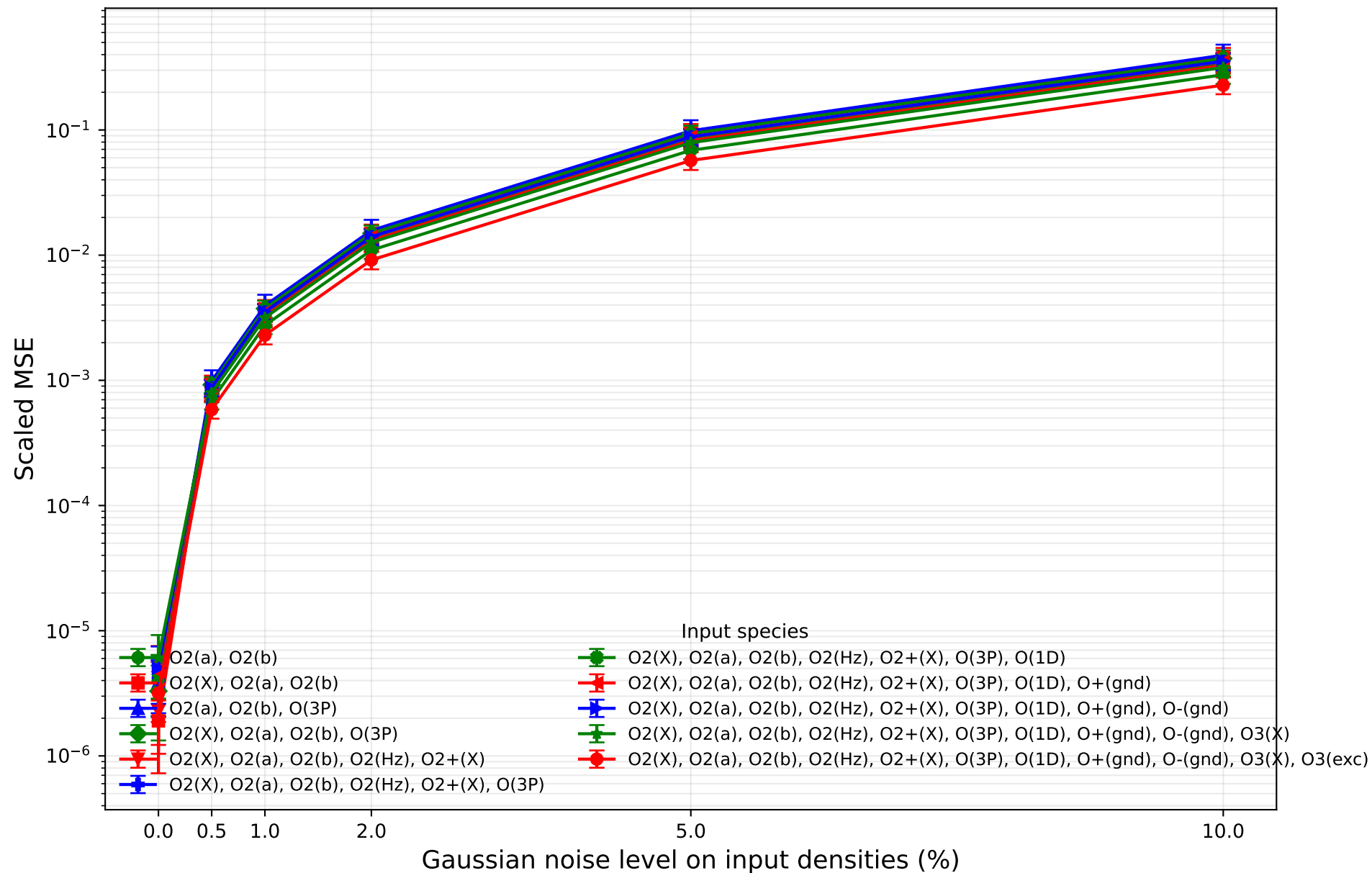
Inverse noise robustness by species configuration Architecture: 30, 30
