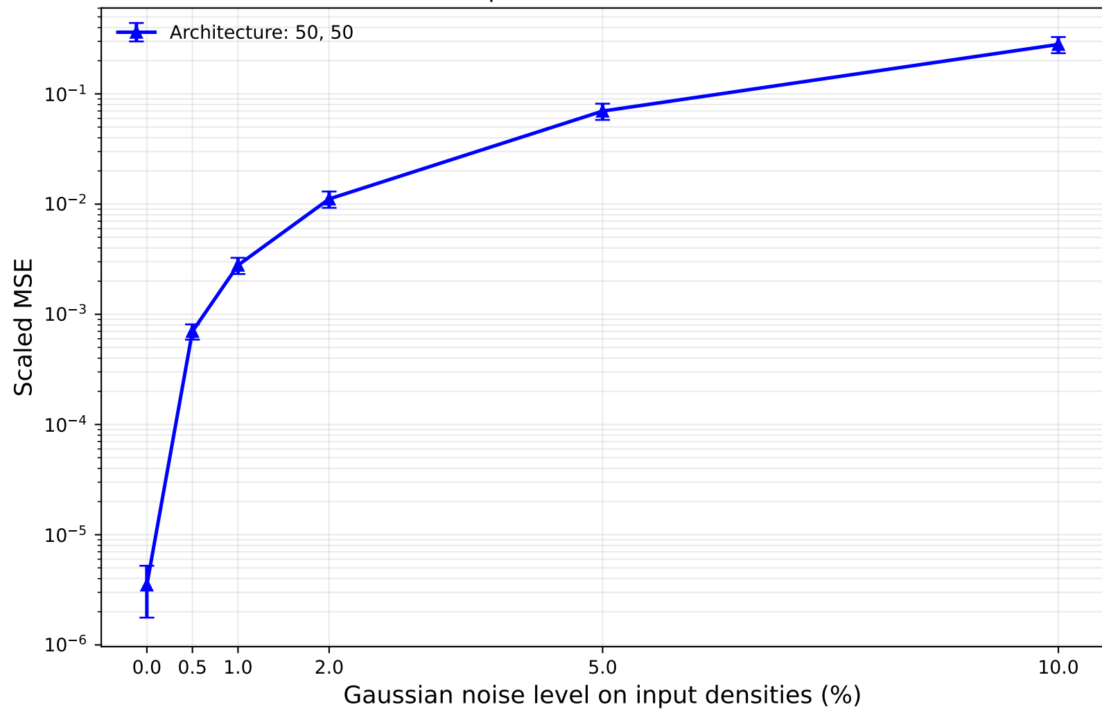
Inverse noise robustness | Architecture: 50, 50 Species: O2(a), O2(b)
