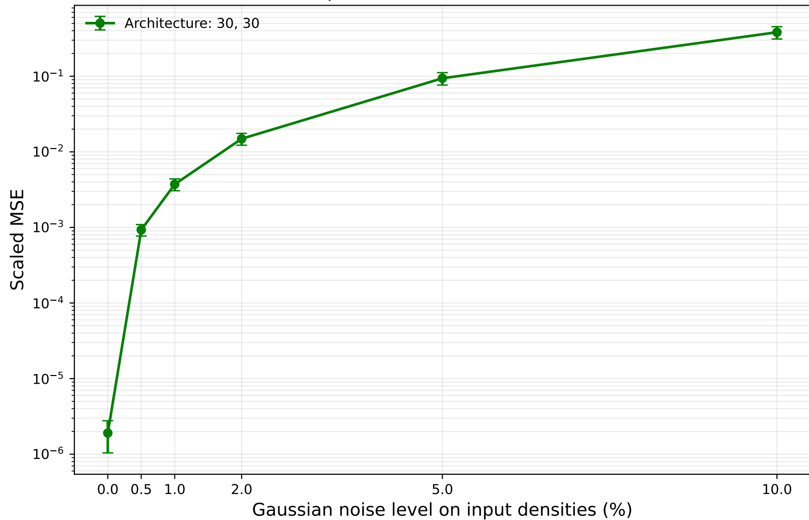
Inverse noise robustness | Architecture: 30, 30 Species: O2(X), O2(a), O2(b)
