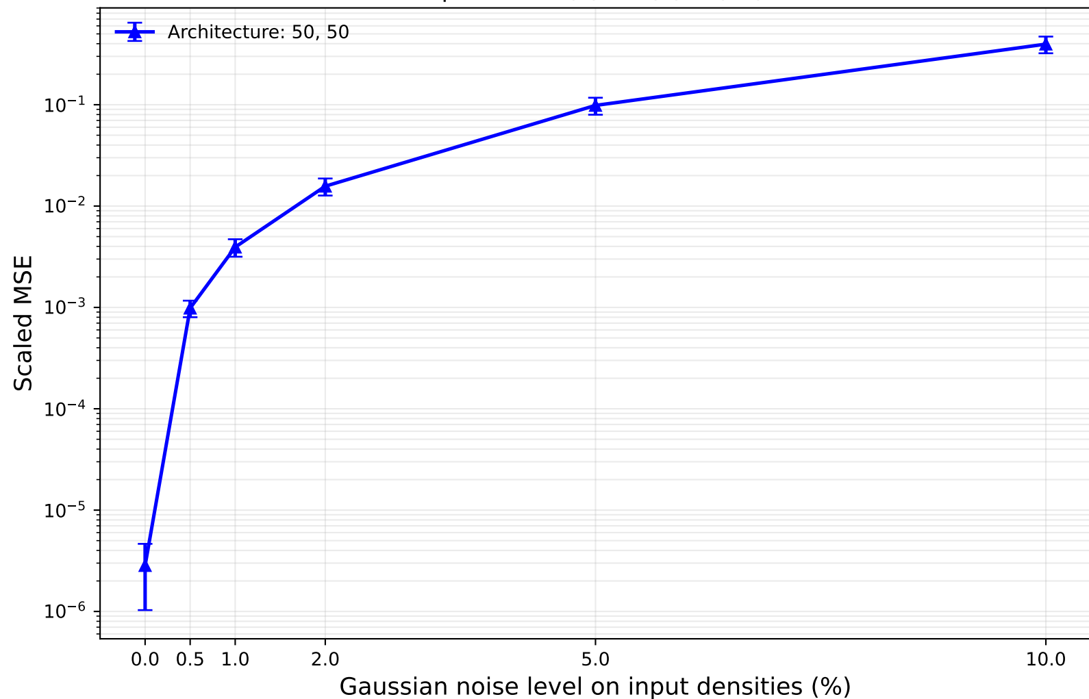
Inverse noise robustness | Architecture: 50, 50 Species: O2(a), O2(b), O(3P)
