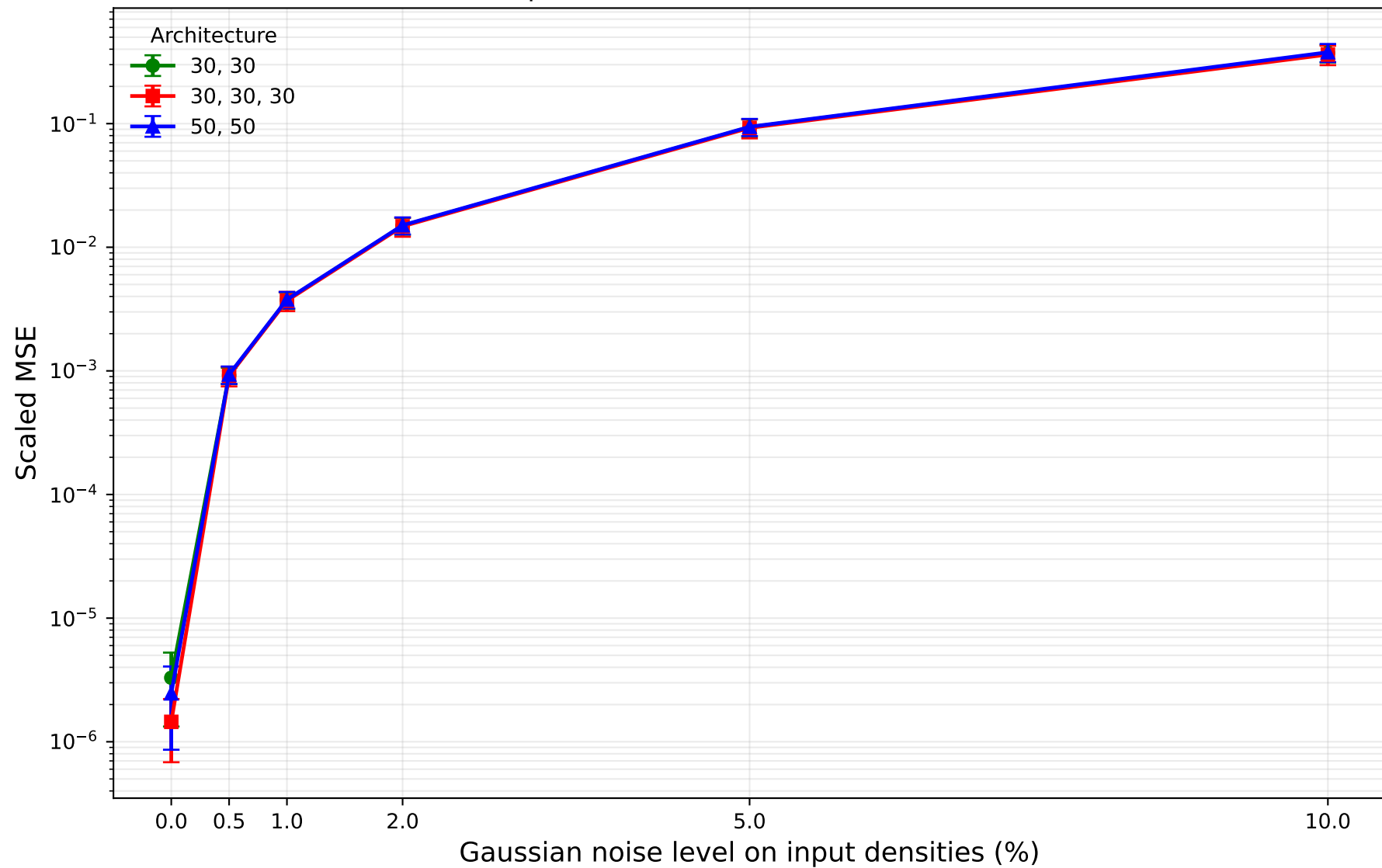
Inverse noise robustness by architecture Species: O2(X), O2(a), O2(b), O(3P)
