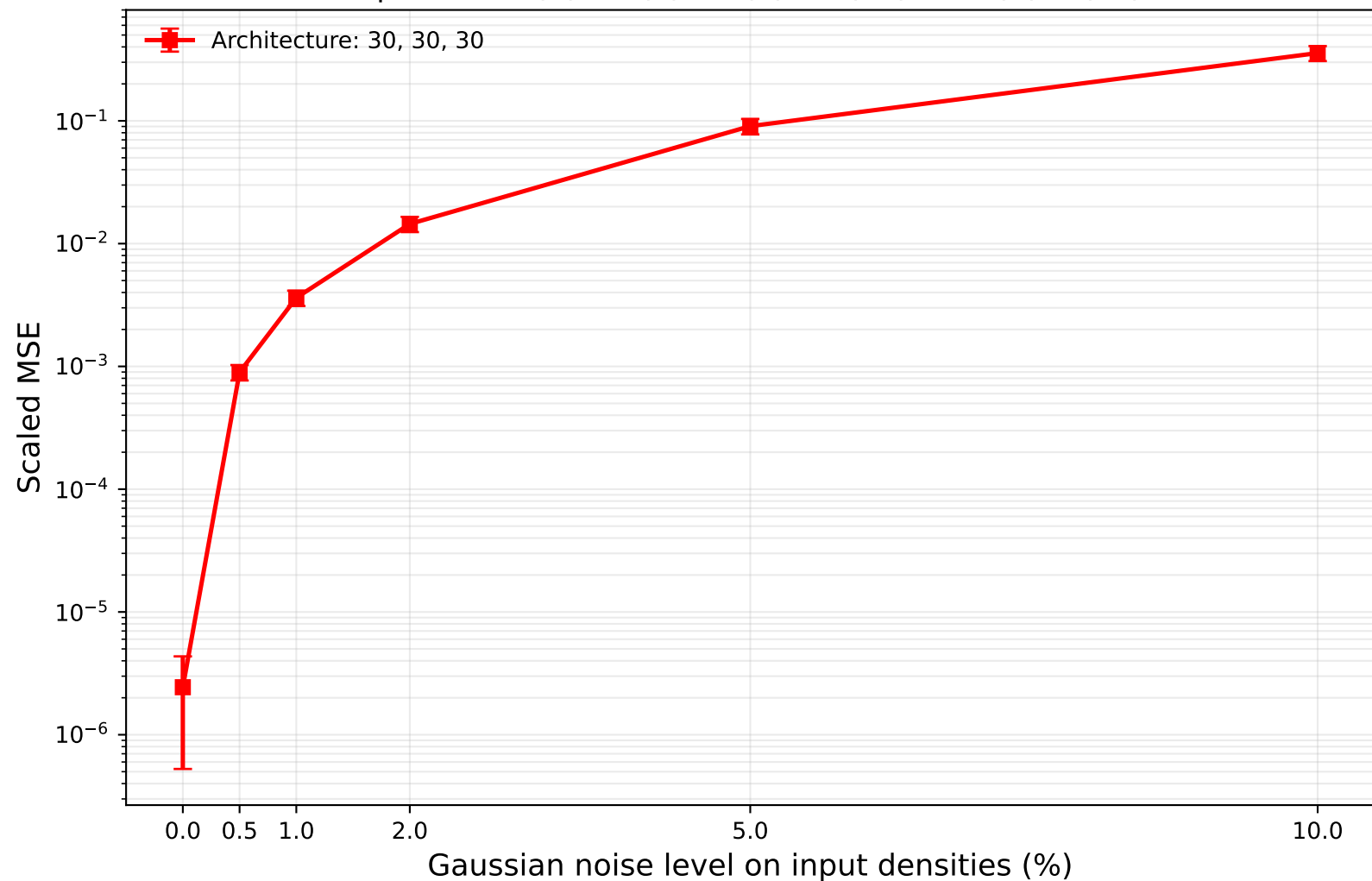
Inverse noise robustness | Architecture: 30, 30, 30 Species: O2(X), O2(a), O2(b), O2(Hz), O2+(X), O(3P)
