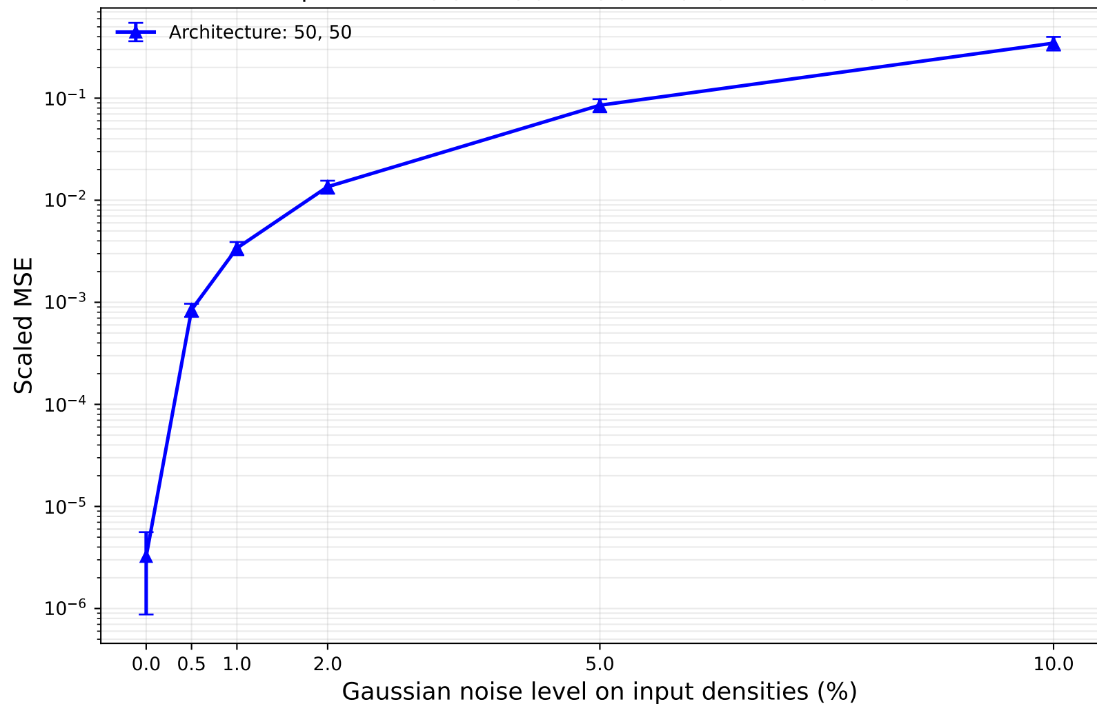
Inverse noise robustness | Architecture: 50, 50 Species: O2(X), O2(a), O2(b), O2(Hz), O2+(X), O(3P)
