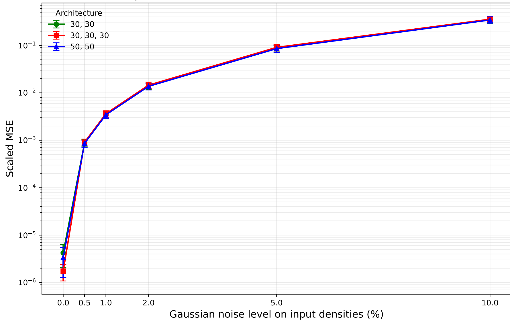
Inverse noise robustness by architecture Species: O2(X), O2(a), O2(b), O2(Hz), O2+(X), O(3P), O(1D)
