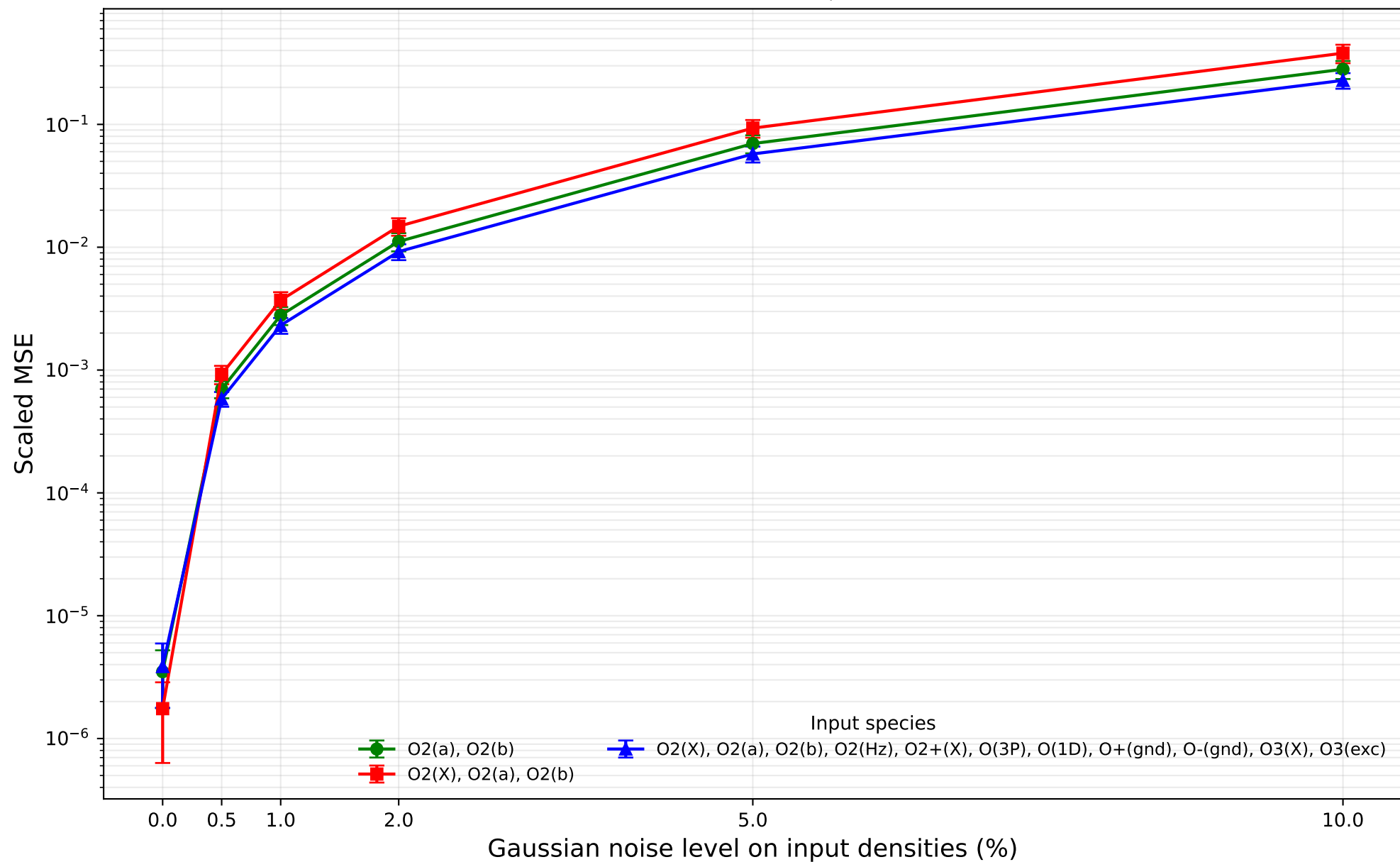
Inverse noise robustness by species configuration Architecture: 50, 50
