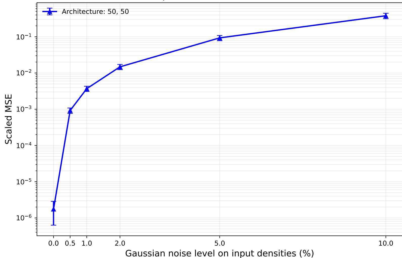
Inverse noise robustness | Architecture: 50, 50 Species: O2(X), O2(a), O2(b)
