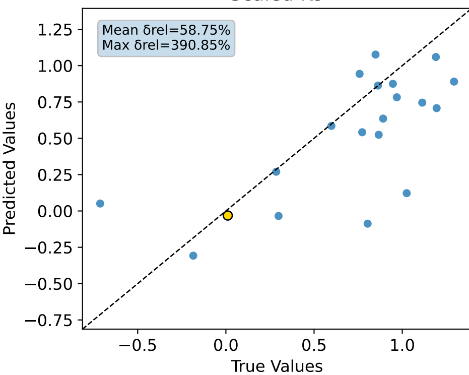
Scaled K9
