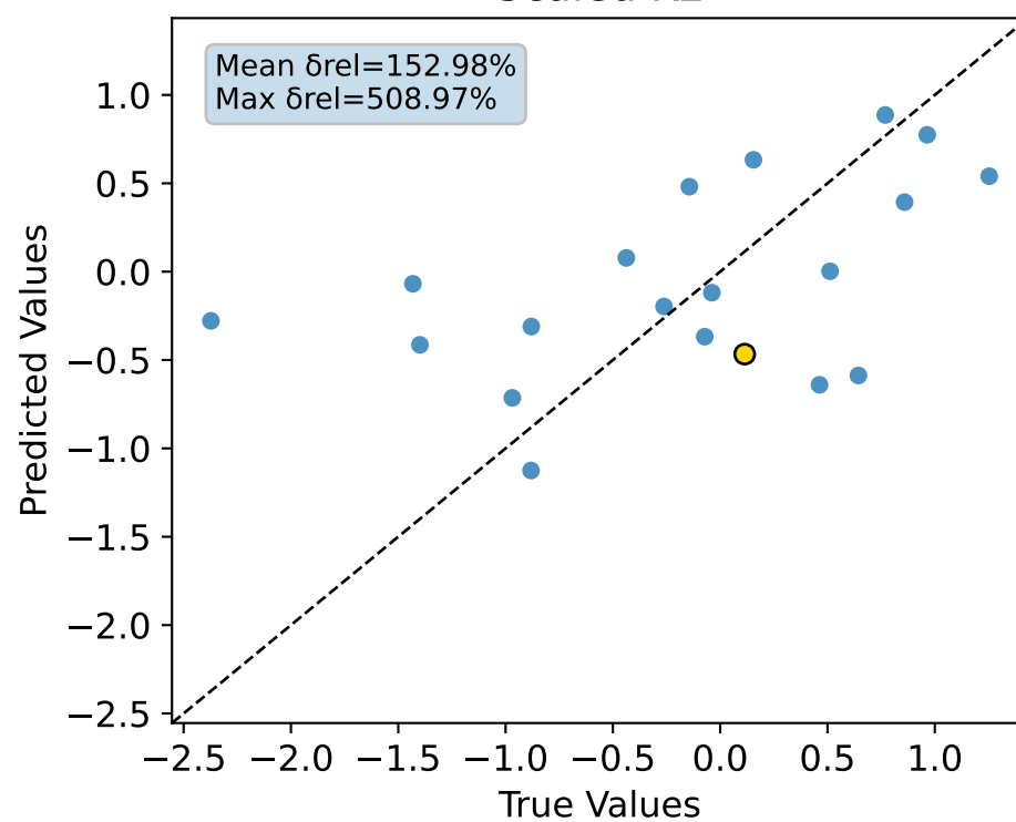
Scaled K5
