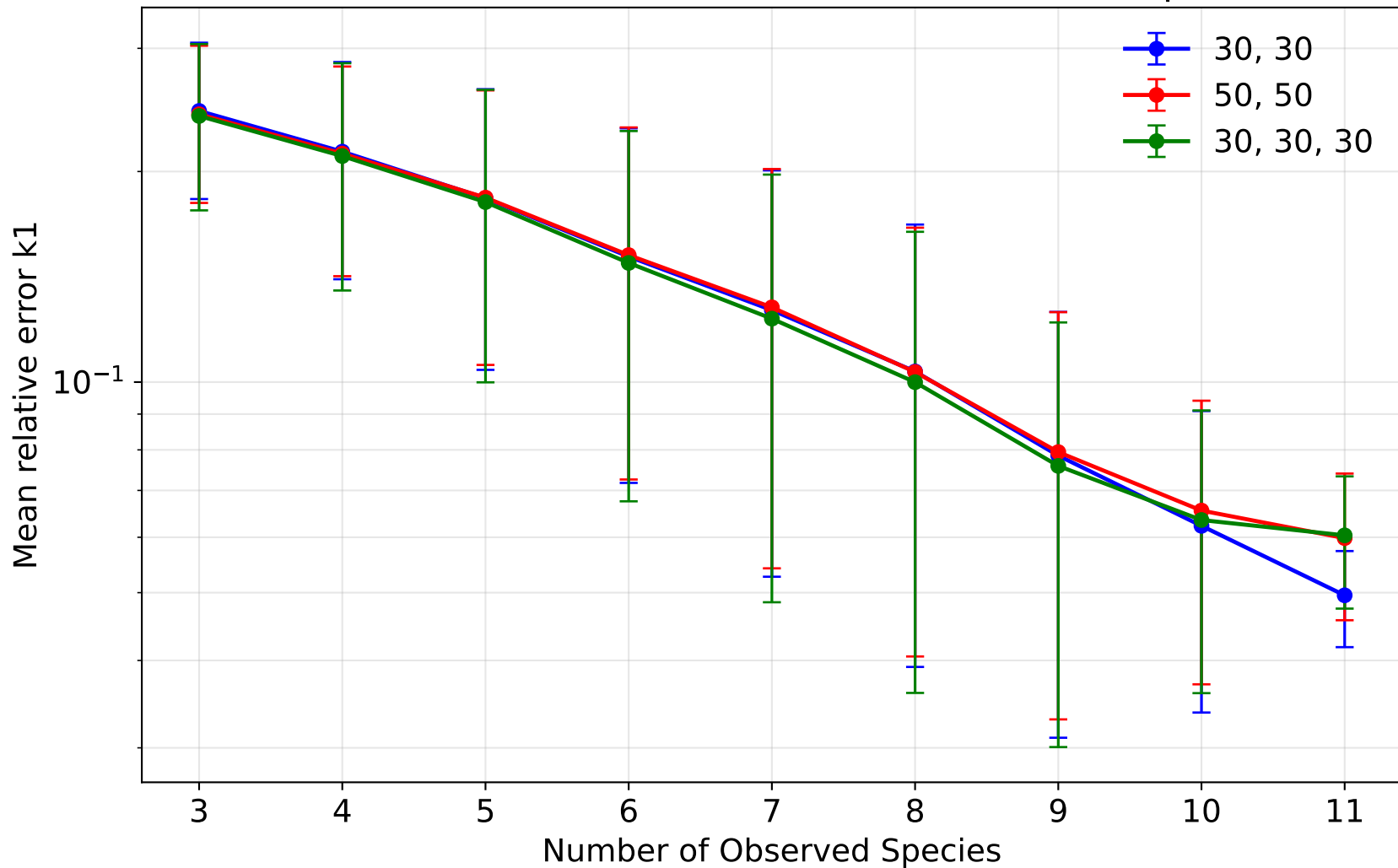
Mean relative error k1 vs number of observed species
