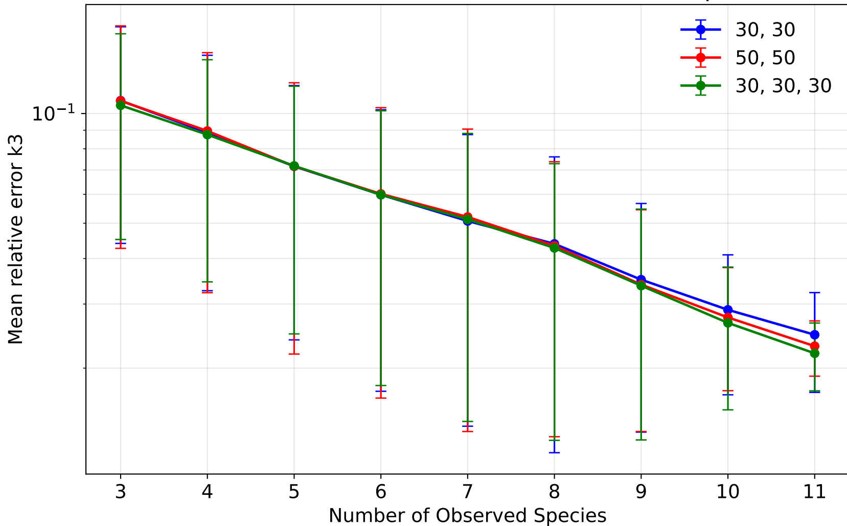
Mean relative error k3 vs number of observed species
