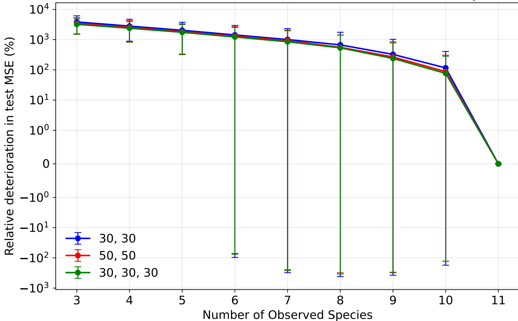
Relative deterioration in test MSE vs number of observed species
