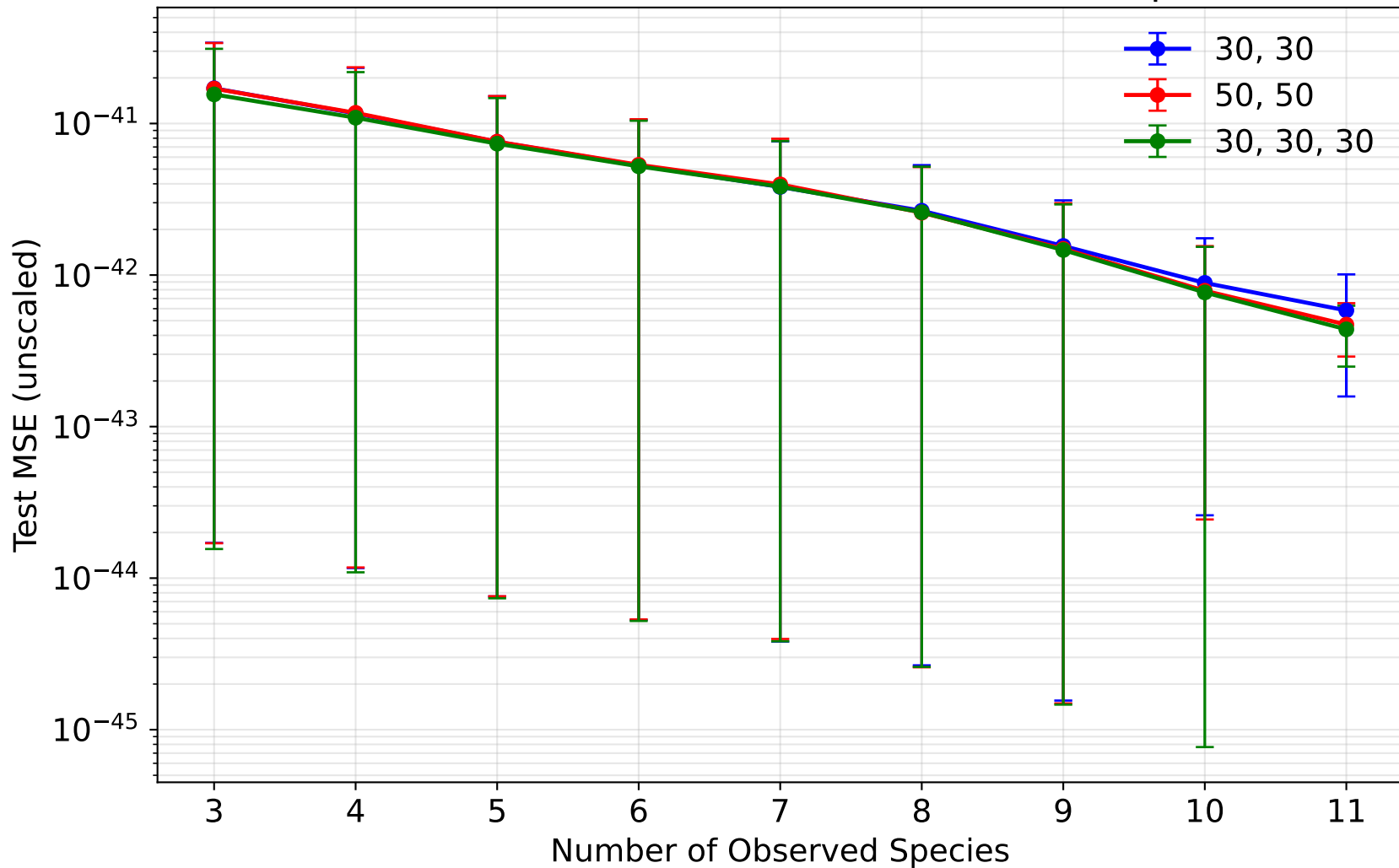
Test MSE (unscaled) vs number of observed species
