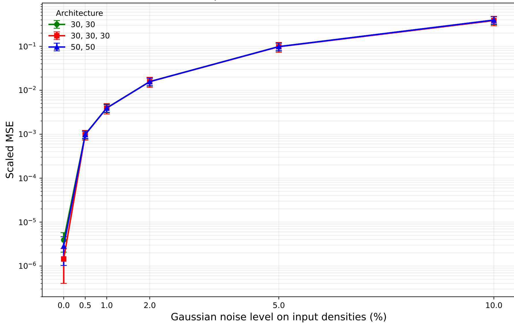
Inverse noise robustness by architecture Species: O2(a), O2(b), O(3P)
