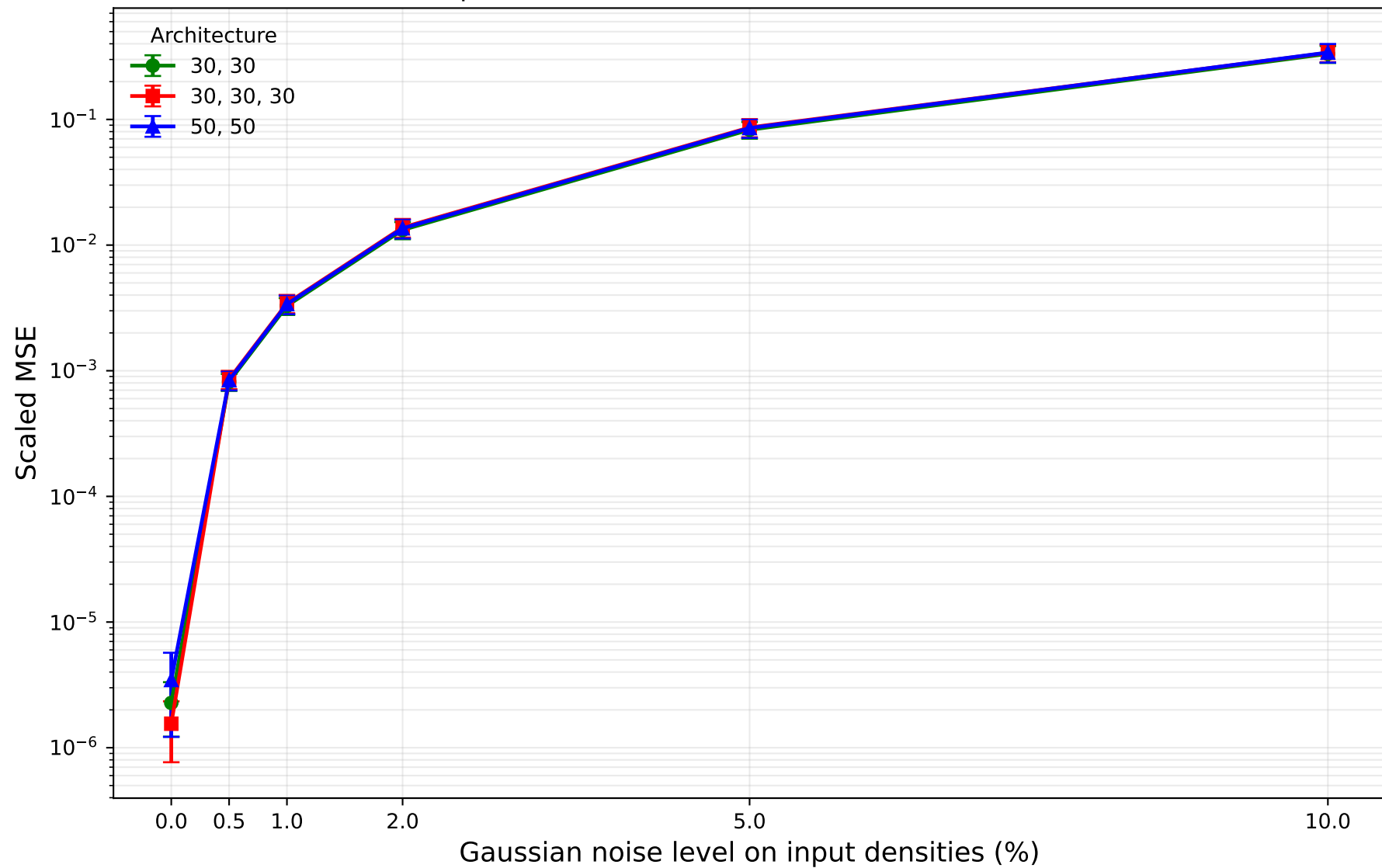
Inverse noise robustness by architecture Species: O2(X), O2(a), O2(b), O2(Hz), O2+(X)
