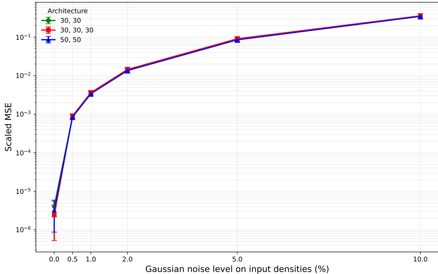
Inverse noise robustness by architecture Species: O2(X), O2(a), O2(b), O2(Hz), O2+(X), O(3P)
