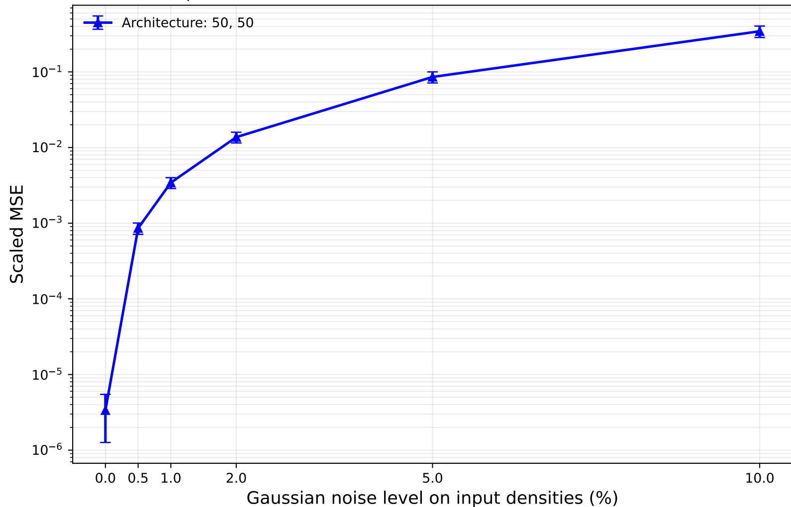
Inverse noise robustness | Architecture: 50, 50 Species: O2(X), O2(a), O2(b), O2(Hz), O2+(X), O(3P), O(1D)
