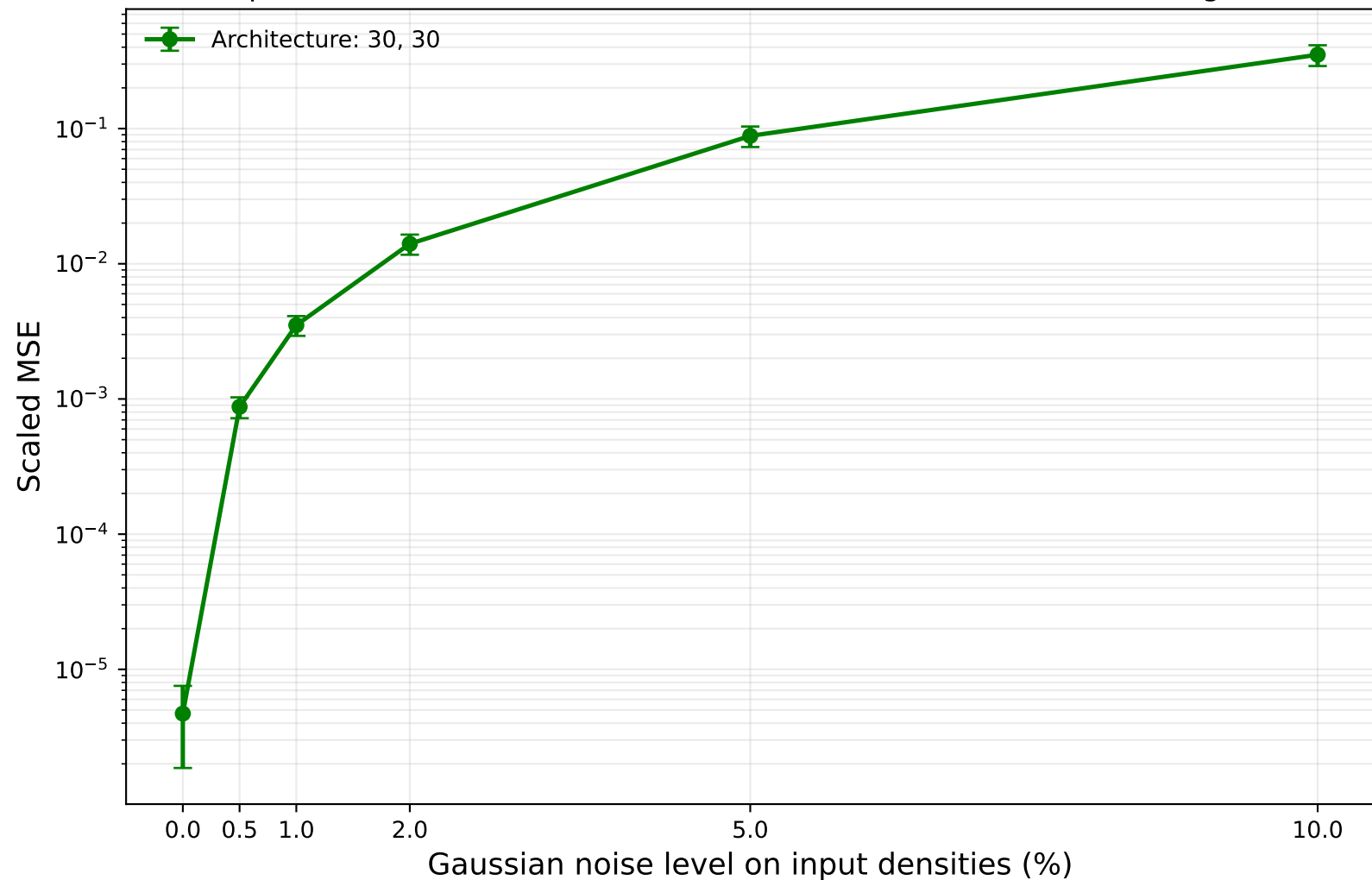
Inverse noise robustness | Architecture: 30, 30 Species: O2(X), O2(a), O2(b), O2(Hz), O2+(X), O(3P), O(1D), O+(gnd)
