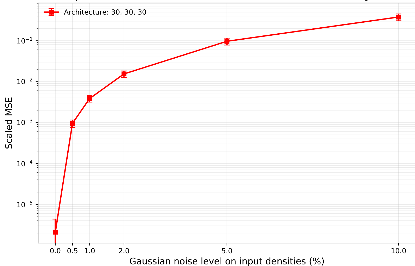
Inverse noise robustness | Architecture: 30, 30, 30 Species: O2(X), O2(a), O2(b), O2(Hz), O2+(X), O(3P), O(1D), O+(gnd)
