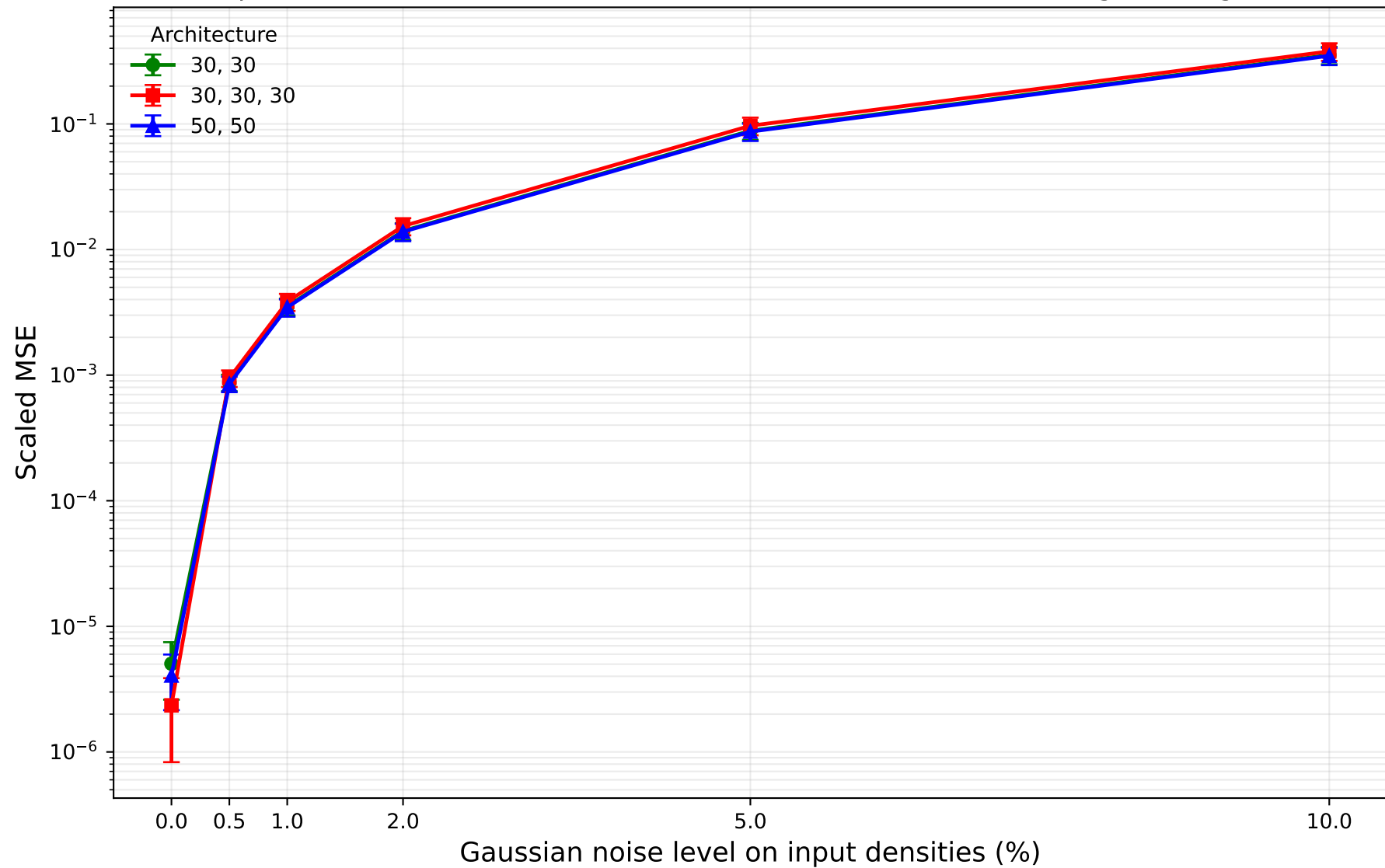
Inverse noise robustness by architecture Species: O2(X), O2(a), O2(b), O2(Hz), O2+(X), O(3P), O(1D), O+(gnd), O-(gnd)
