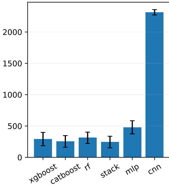
RMSE
