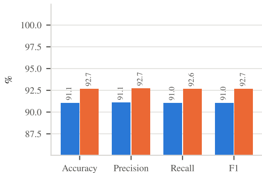
Yelp Full
