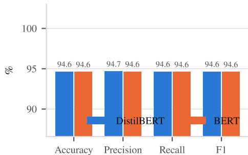
Yelp Polarity
