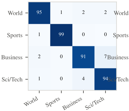
DistilBERT
