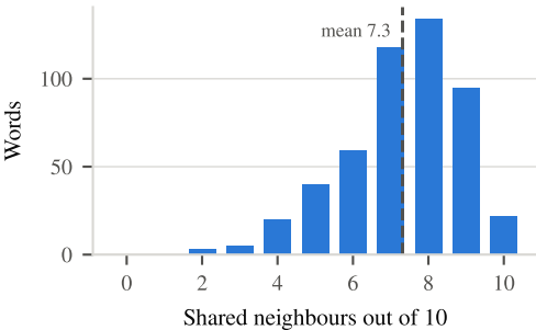
Agreement on the closest words
