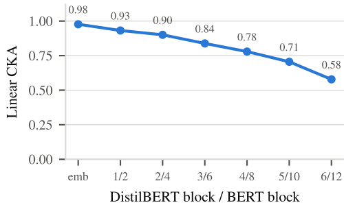
Alignment falls with depth
