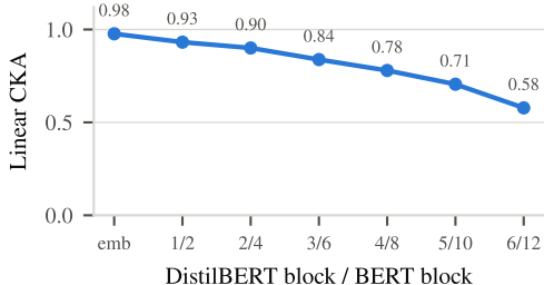
Alignment falls with depth
