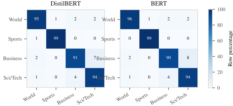
Figure 3: Row normalised confusion matrices on AG News. The two models make the same kind of mistake in the same place.
