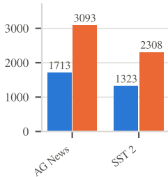
Peak GPU memory training (MiB)
