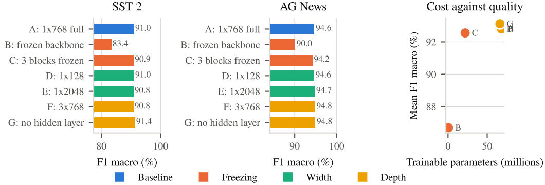
Figure 3: Classifier ablation on DistilBERT. Left and centre: F1 macro per variant. Right: trainable parameters against mean F1 macro.
