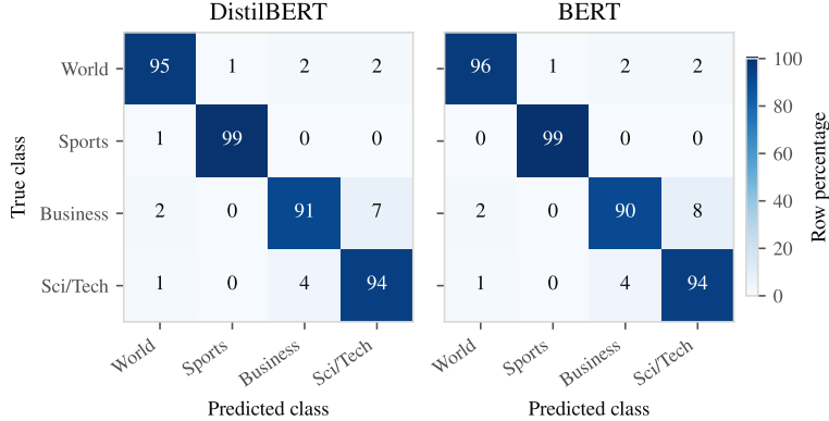
Figure 3: Row normalised confusion matrices on AG News. The two models make the same kind of mistake in the same place.
