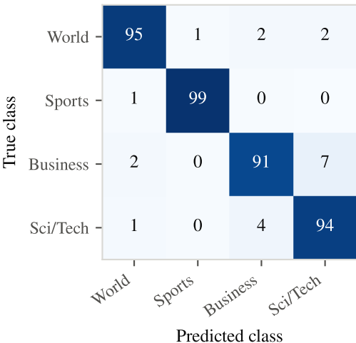
DistilBERT
