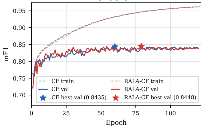
S2Looking
