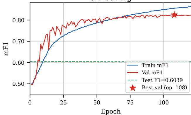
S2Looking
