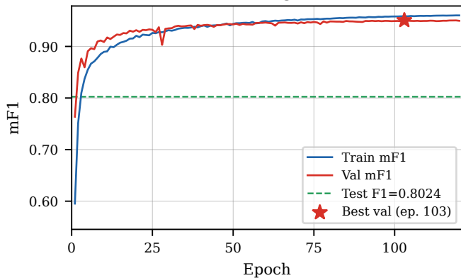
WHU-CD
