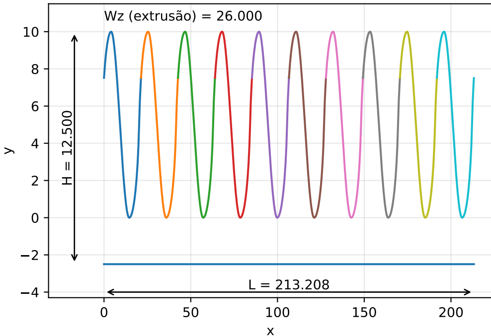
2D profile with main dimensions
