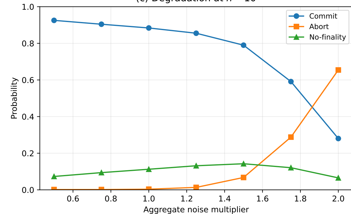
(c) Degradation at n = 10
