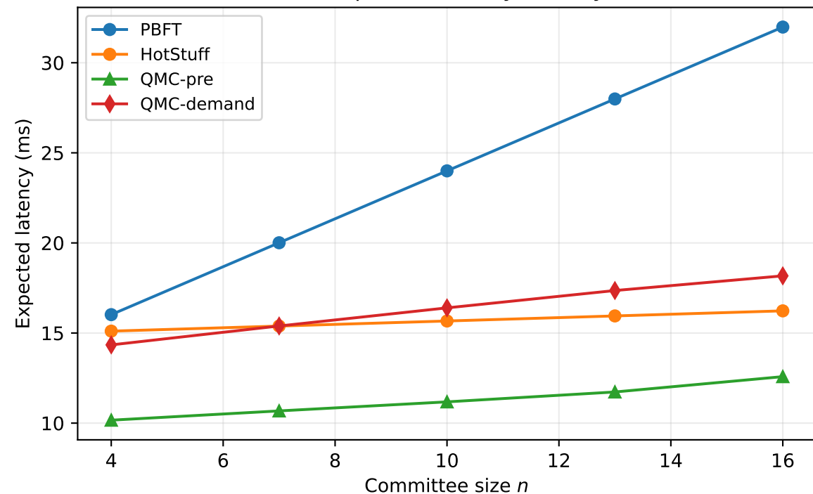
(b) Expected finality latency
