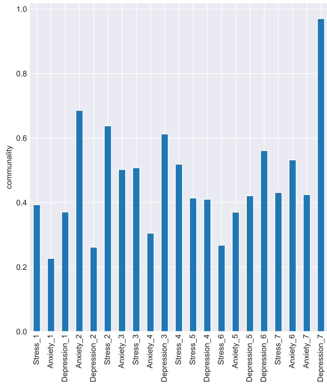
Oblimin Rotation
