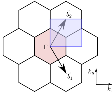
Figure 4.3: Rectangle with an equivalent area to the BZ for a 2D hexagonal lattice.
