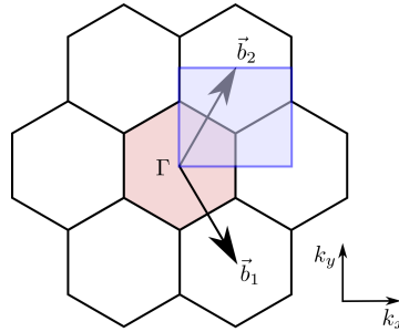
Figure 4.3: Rectangle with an equivalente area to the BZ for a 2D hexagonal lattice.
