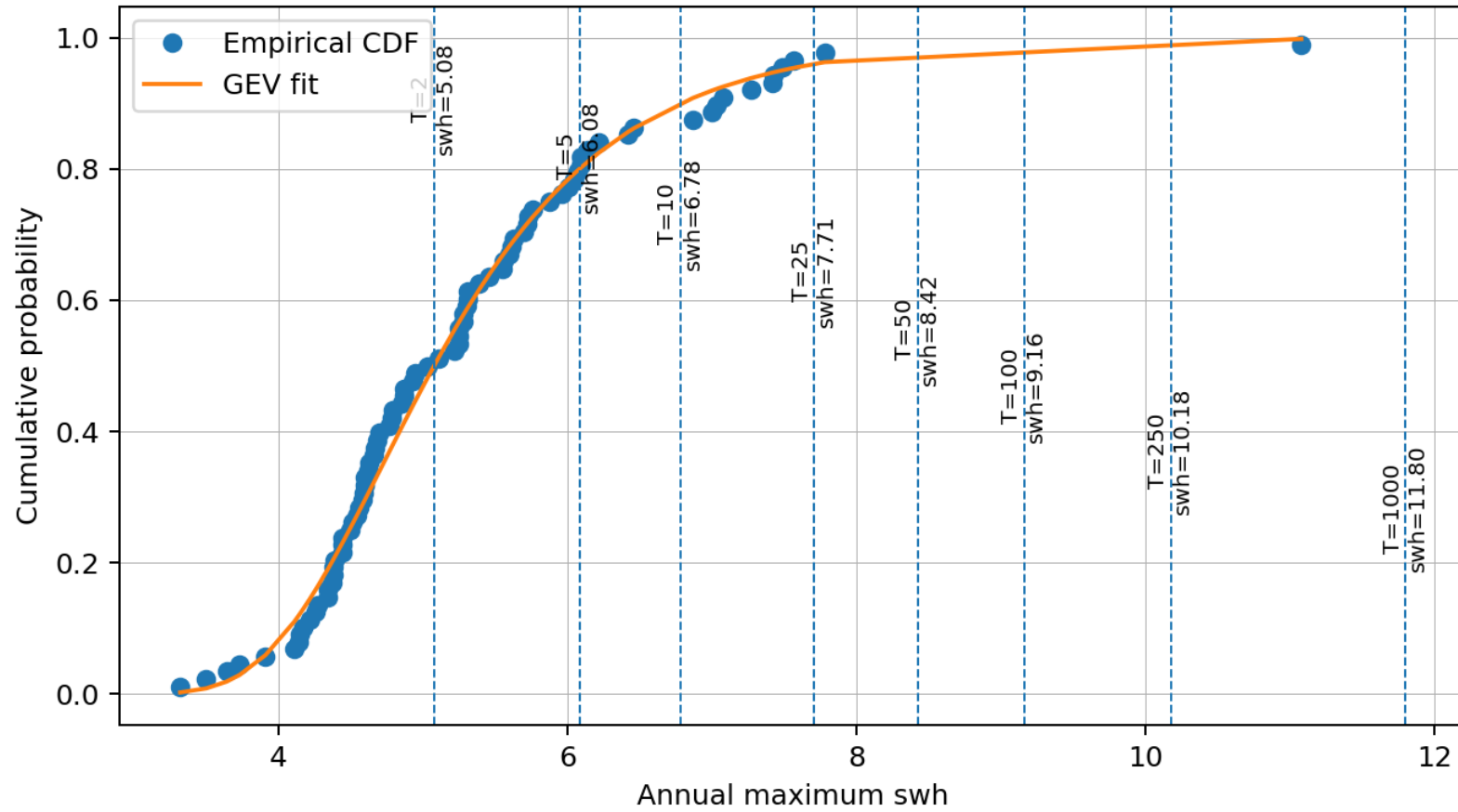
GEV fit: SWH - 210-240
