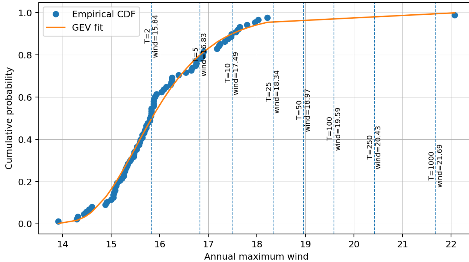
GEV fit: WIND - 000-030
