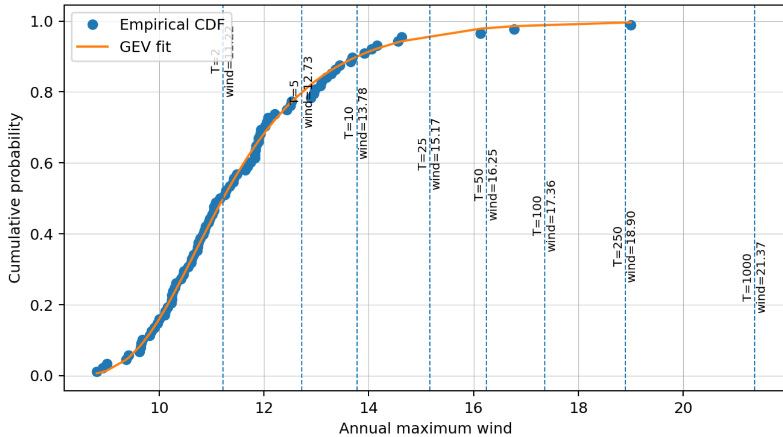
GEV fit: WIND - 090-120
