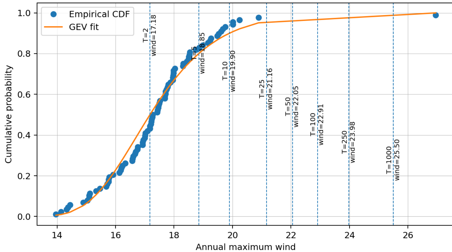
GEV fit: WIND - 210-240
