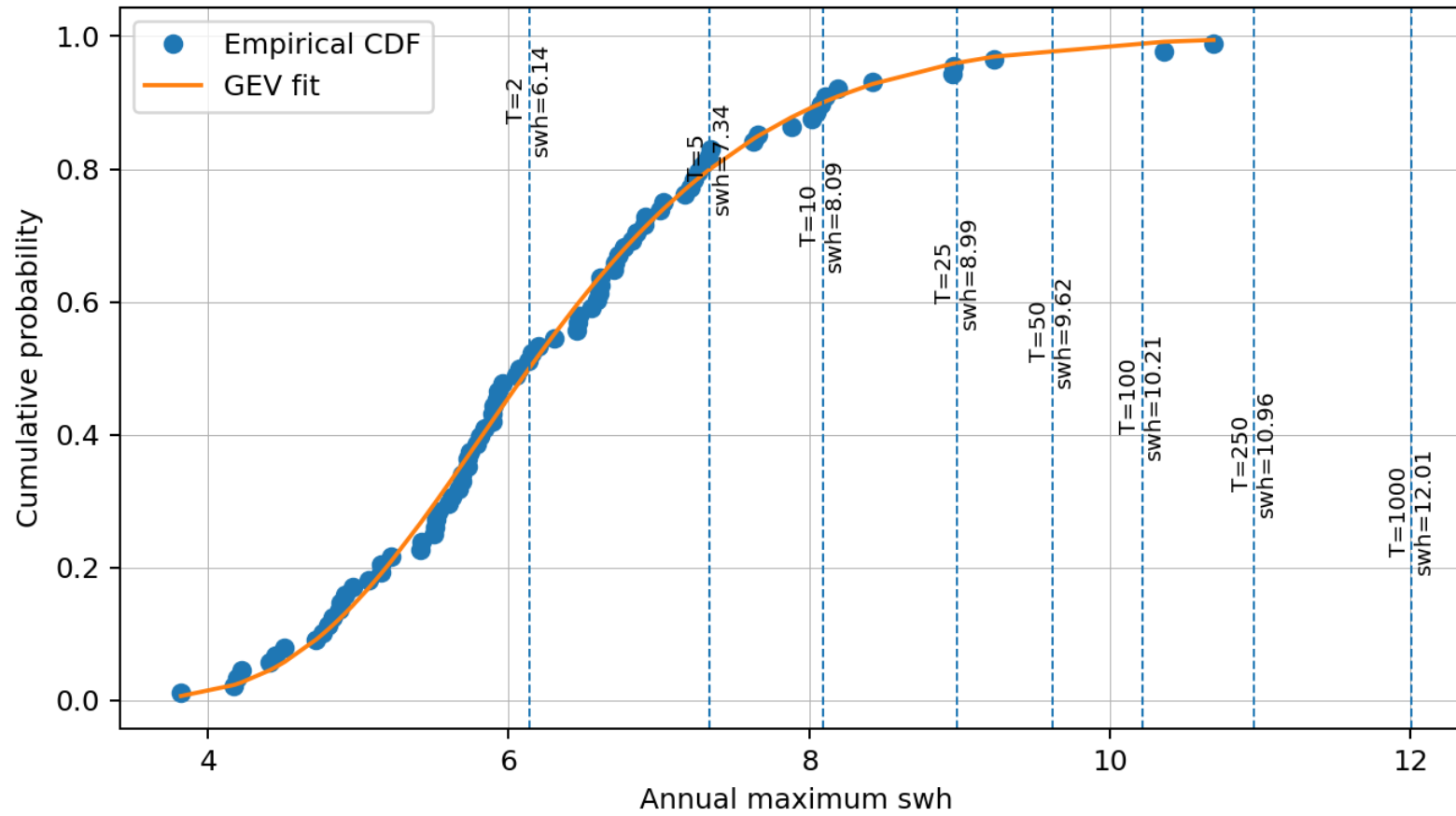
GEV fit: SWH - 240-270
