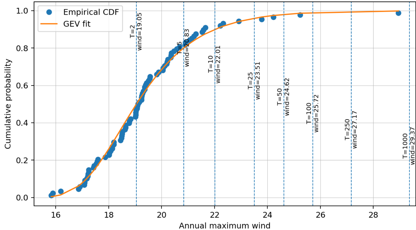
GEV fit: WIND - all directions
