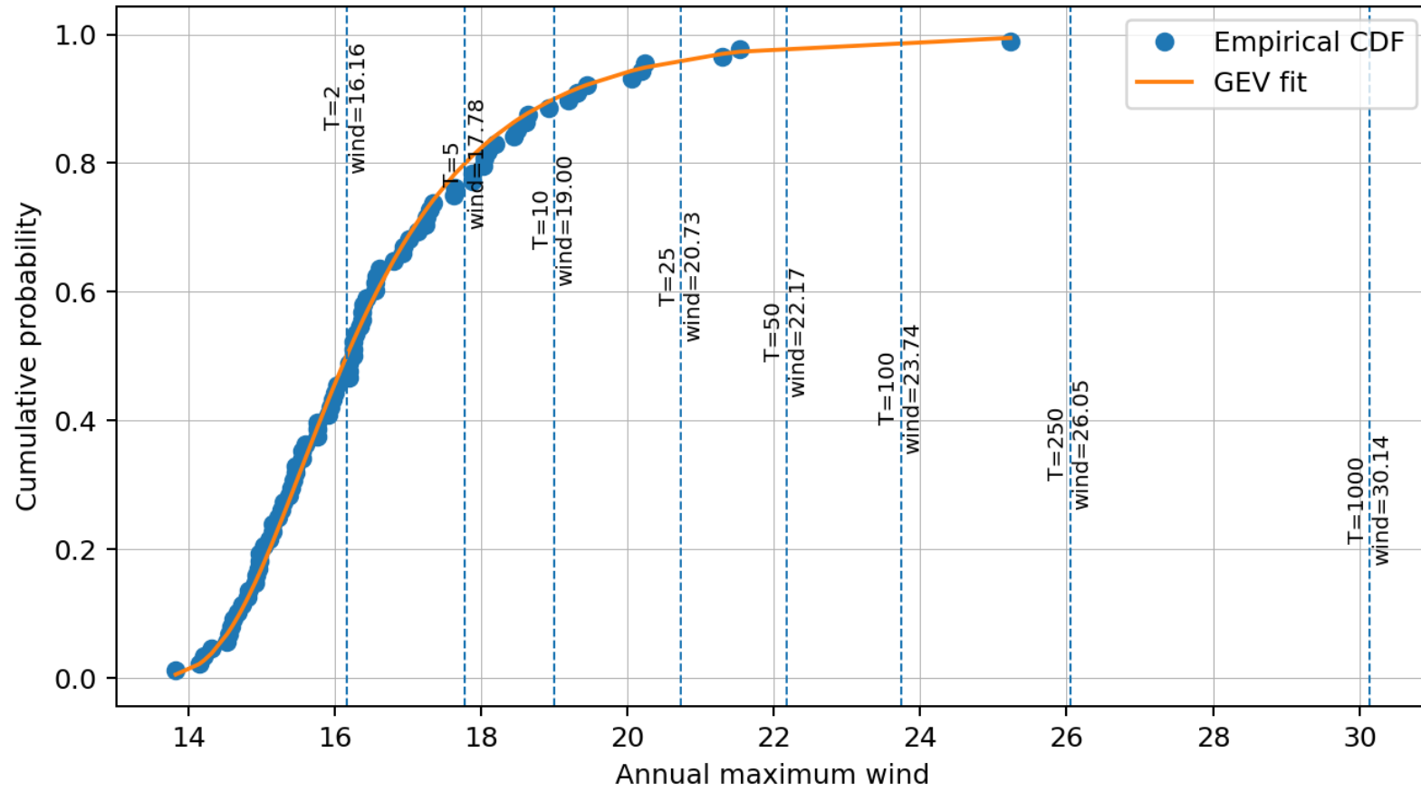
GEV fit: WIND - 330-360
