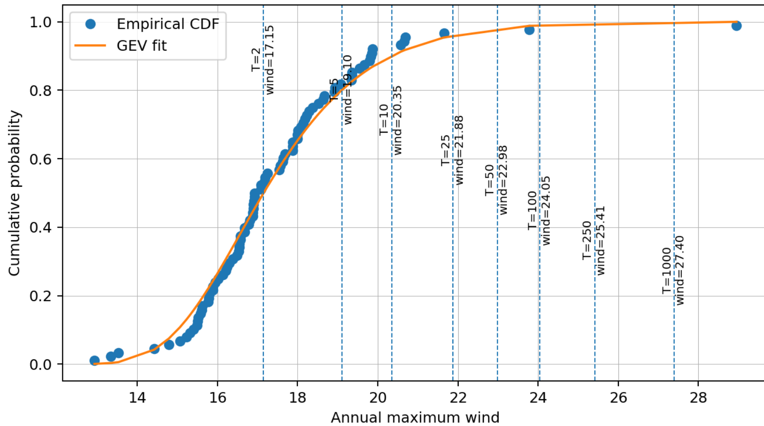
GEV fit: WIND - 150-180
