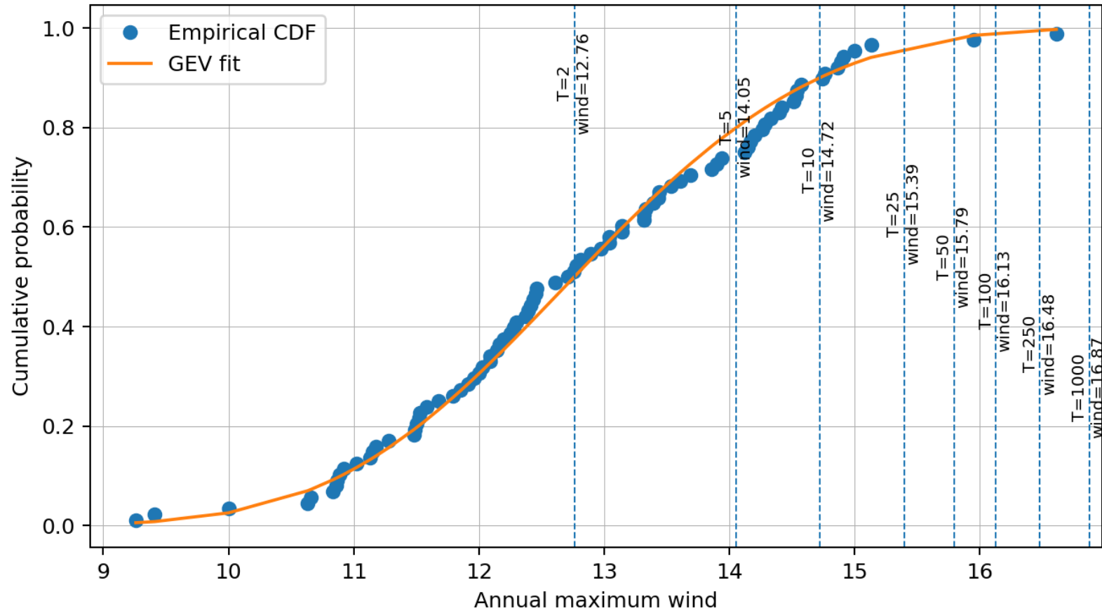
GEV fit: WIND - 030-060
