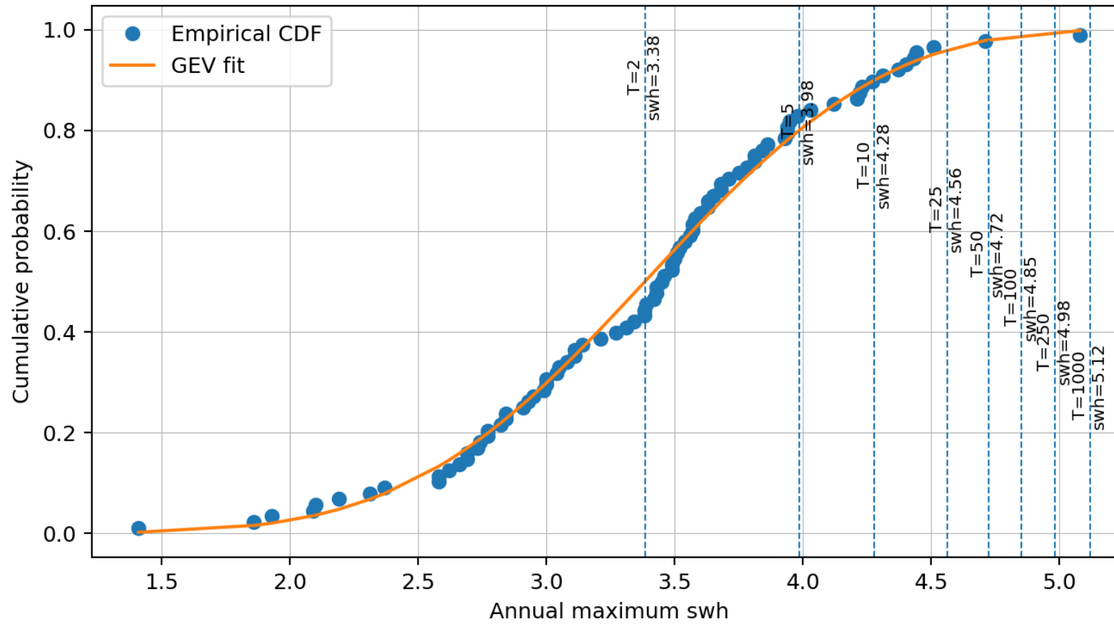
GEV fit: SWH - 000-030
