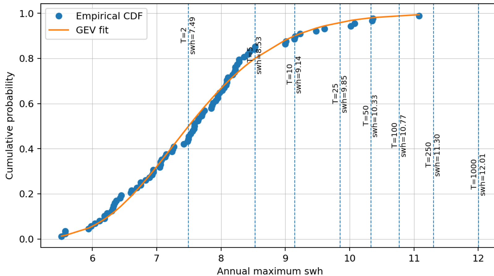
GEV fit: SWH - all directions
