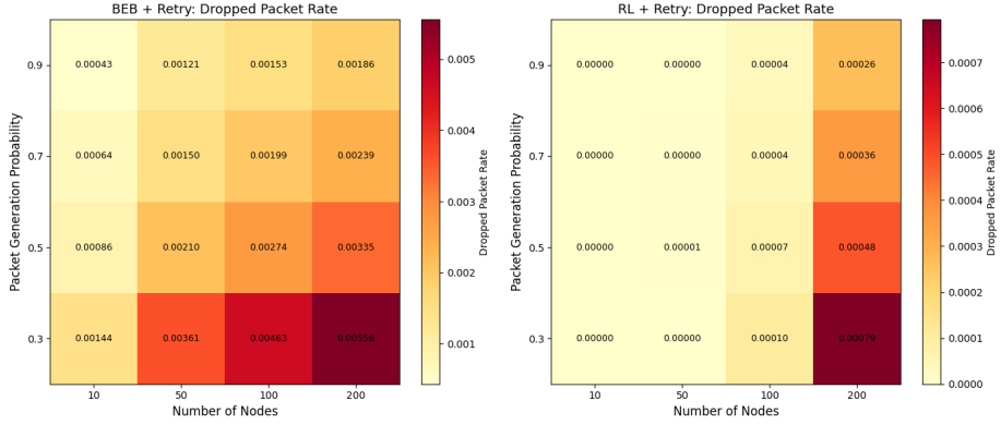
Figure 6: Retry Limit Impact: Dropped Packet Rate Heatmap
