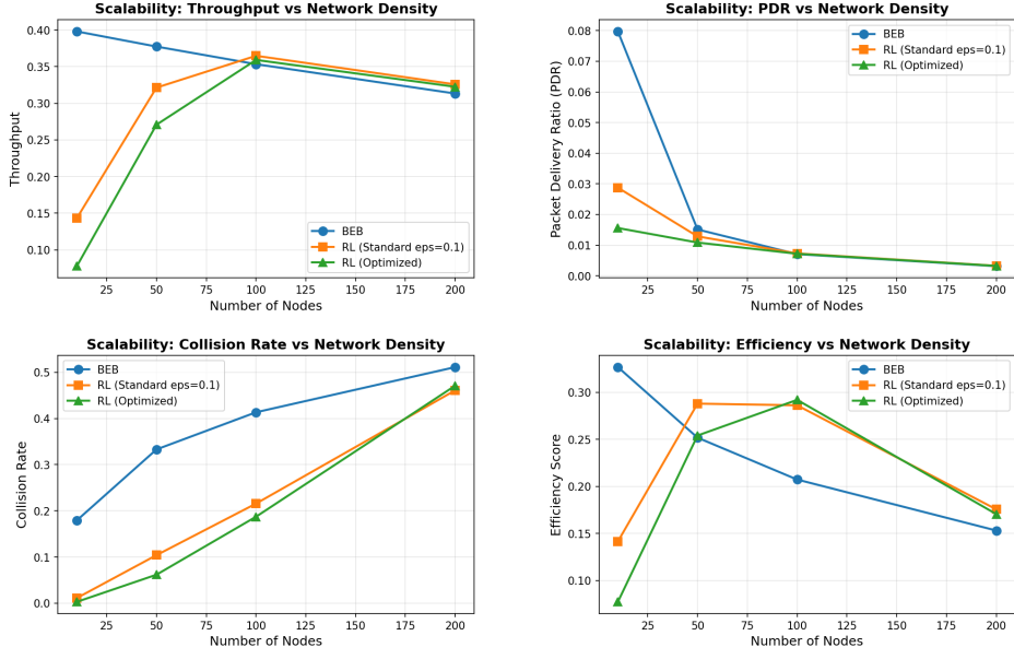
Figure 3: a Scalability Analysis correlated with Throughput, PDR, and Collision Rate vs. Network Density (10-seed averaged). RL (Optimized) uses epsilon decay ( \epsilon : 1.0 \rightarrow 0.01 ), while RL (Standard) uses fixed \epsilon = 0.1 .
