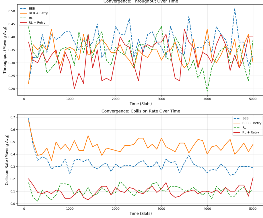
Figure 5: Convergence Analysis with Retry Limits: Throughput and Collision Rate
