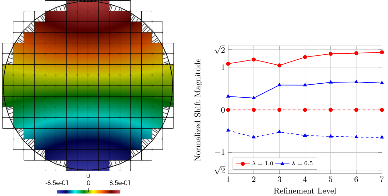
Figure 3: Left: Exemplary numerical solution for the Poisson equation on a unit ball, visualized on the surrogate domain ( \lambda = 0.75 ), obtained with the shifted boundary method. The true boundary \Gamma is shown in black lines; connections between quadrature points ( p = 2 ) on the surrogate boundary and their projections on the true boundary are illustrated with grey lines. Note that with \lambda = 0.75 , some parts of the true boundary lie within the surrogate domain. Right: Illustrative distribution of minimum and maximum shift magnitudes (normalized by cell size h ) on the surrogate boundary for the unit ball problem with p = 3 . The values \pm\sqrt{2} represent the theoretical maximum possible normalized shift magnitude in 2D for a square cell. For \lambda = 1.0 the maximum shift magnitude was 1.3510, while for \lambda = 0.5 it was 0.6436 and the minimum -0.6299.
