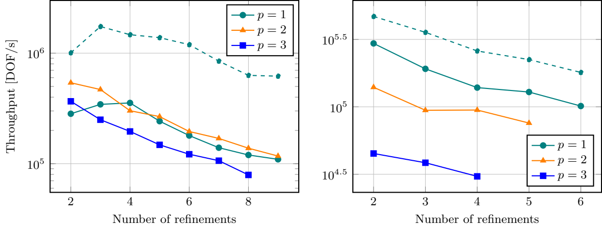
Figure 5: Comparison of throughput (DOF/s) for the proposed multigrid preconditioner with Full-Residual Shy Patch smoother with \xi = 3 , s = 3 (solid line), against an AMG preconditioner (dashed line) from deal.II 's interface to Trilinos . The tests are performed on the unit ball problem in 2D for polynomial degrees p = 1, 2, 3 with s = 3 smoothing steps. Timings obtained on a single core of an AMD EPYC 7282.
