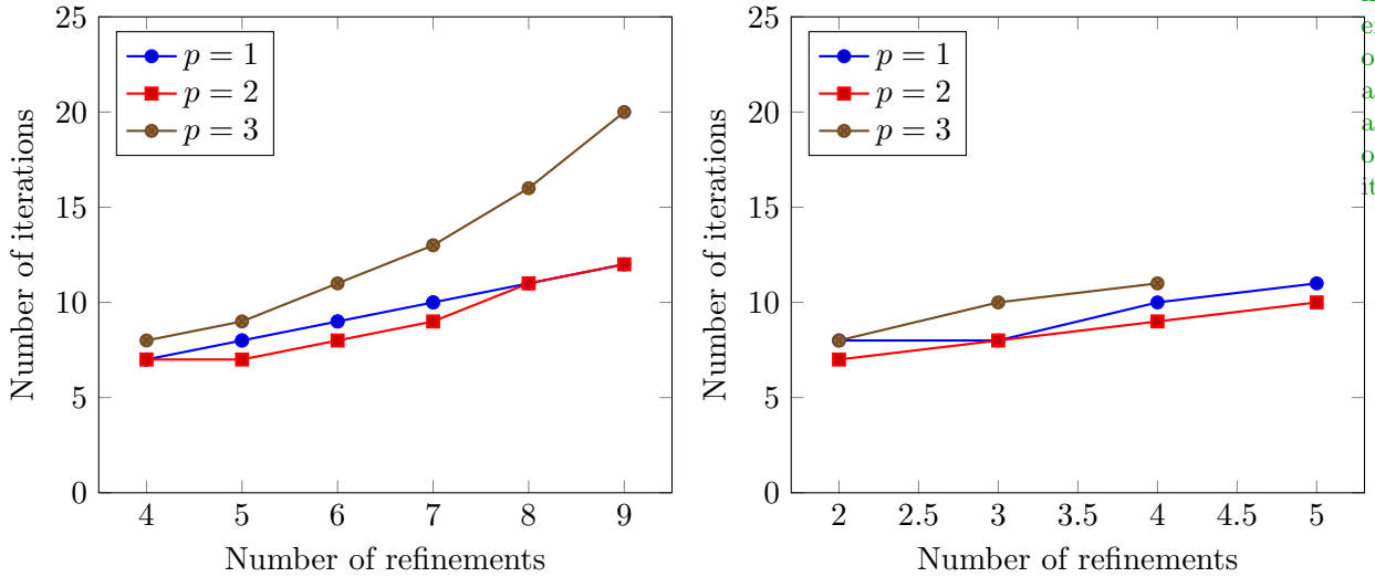
Figure 3: Iteration counts for multigrid preconditioned GMRES solver using the Full-Residual Shy Patch smoother with varying shyness thresholds equal to 3 on unit ball problem for polynomial degrees p = 1, 2, 3 . Number of smoothing steps is fixed to 3. Left panel presents results in 2D, right panel in 3D.
