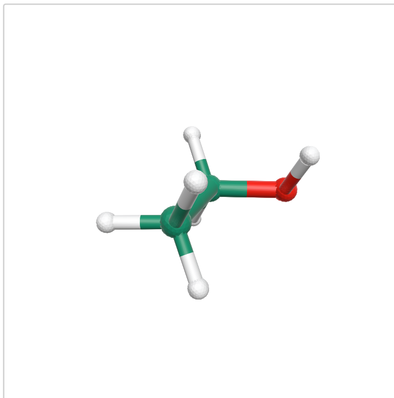
Figure 8: PubChem CID 702 (ethanol) rendered from XYZ with the complete settings above.
