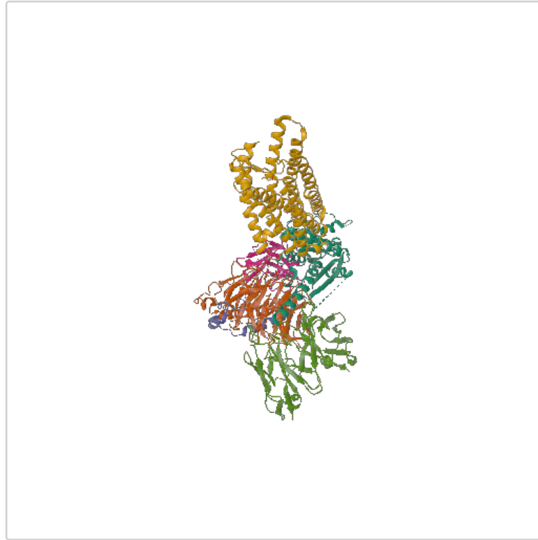
Figure 7: RCSB PDB entry 9M1U rendered as a Cartoon with automatic quality and PNG output.
