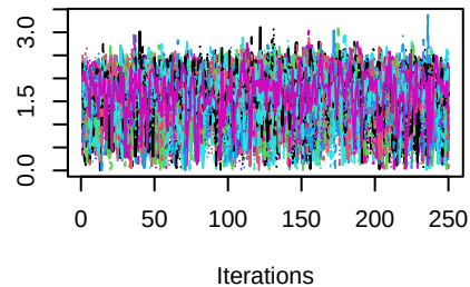
Trace of B.tie.same.h1
