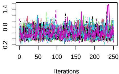
Trace of A.h2
