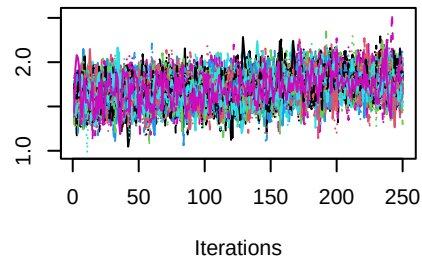
Trace of mean_v.untrained.false.h1
