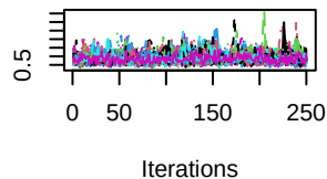
Trace of B.tie.diff.h2
