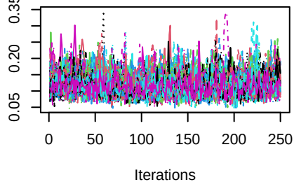
Trace of t0.untrained.h2
