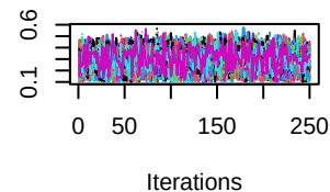
Trace of t0.both.h1
