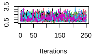
Trace of B.both.same.h2
