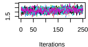
Trace of mean_v.both.false.h
