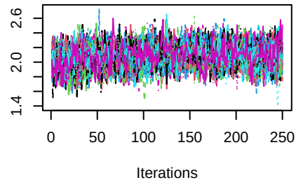
Trace of mean_v.name.false.h1
