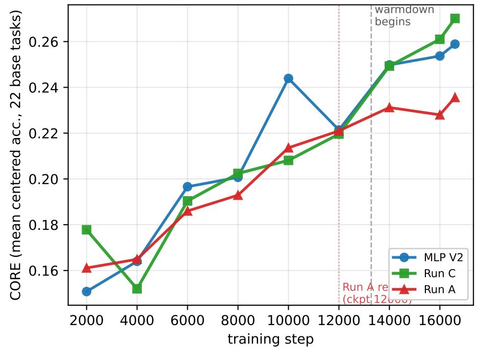
(c) CORE vs step (every 2000 steps; 500/task at final)
