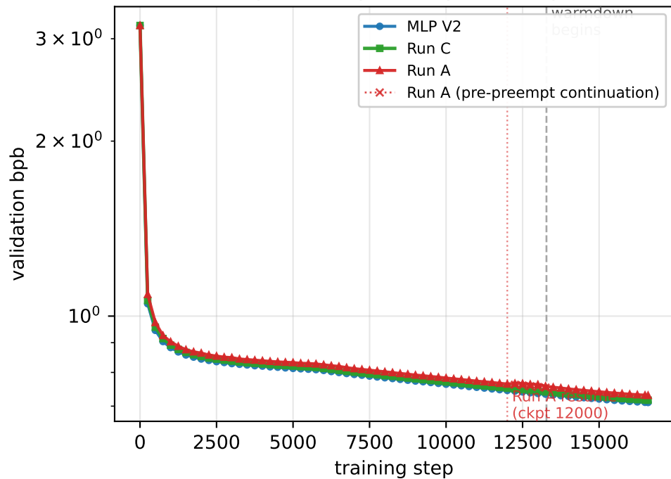
(a) bpb vs step (every 250 steps)
