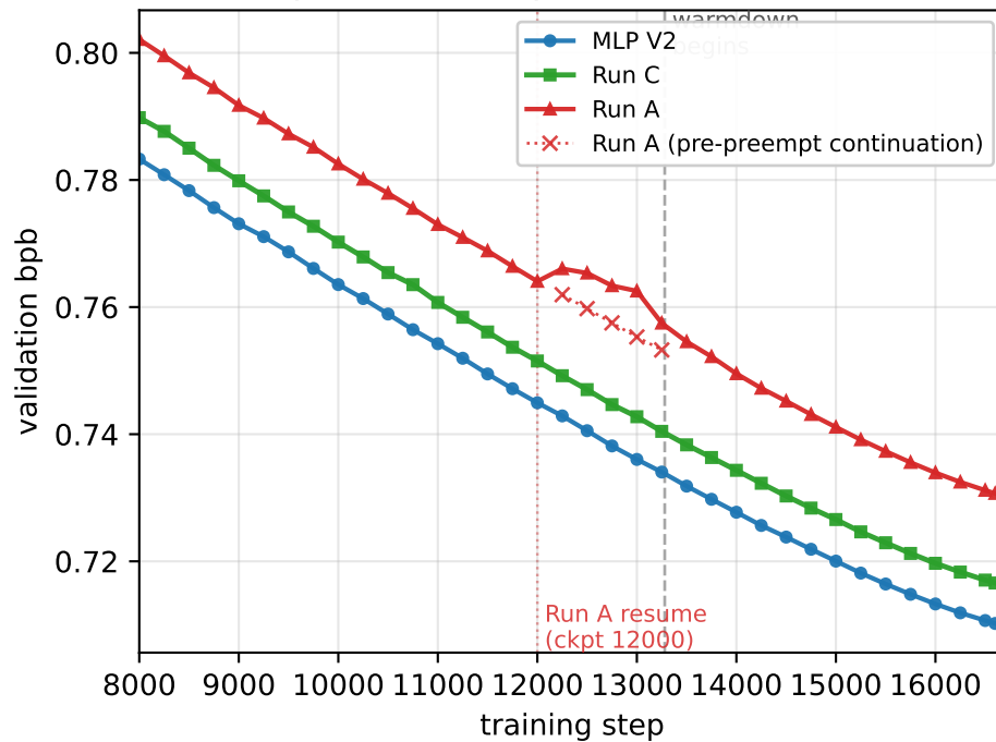
(b) bpb zoom (steps 8000-16600, linear)
