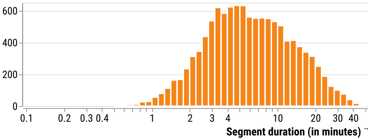
Orthodromy
