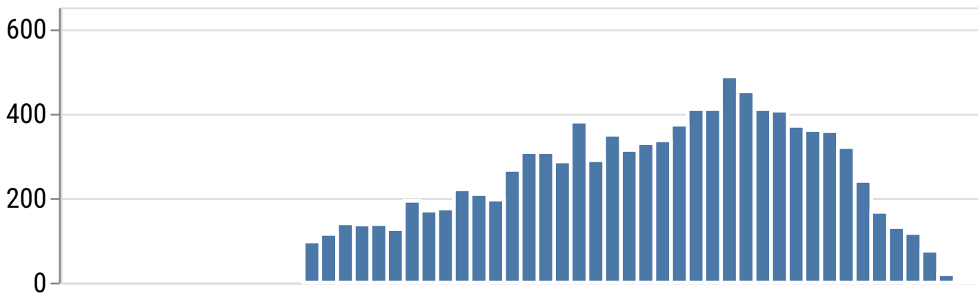
Orthodromy
