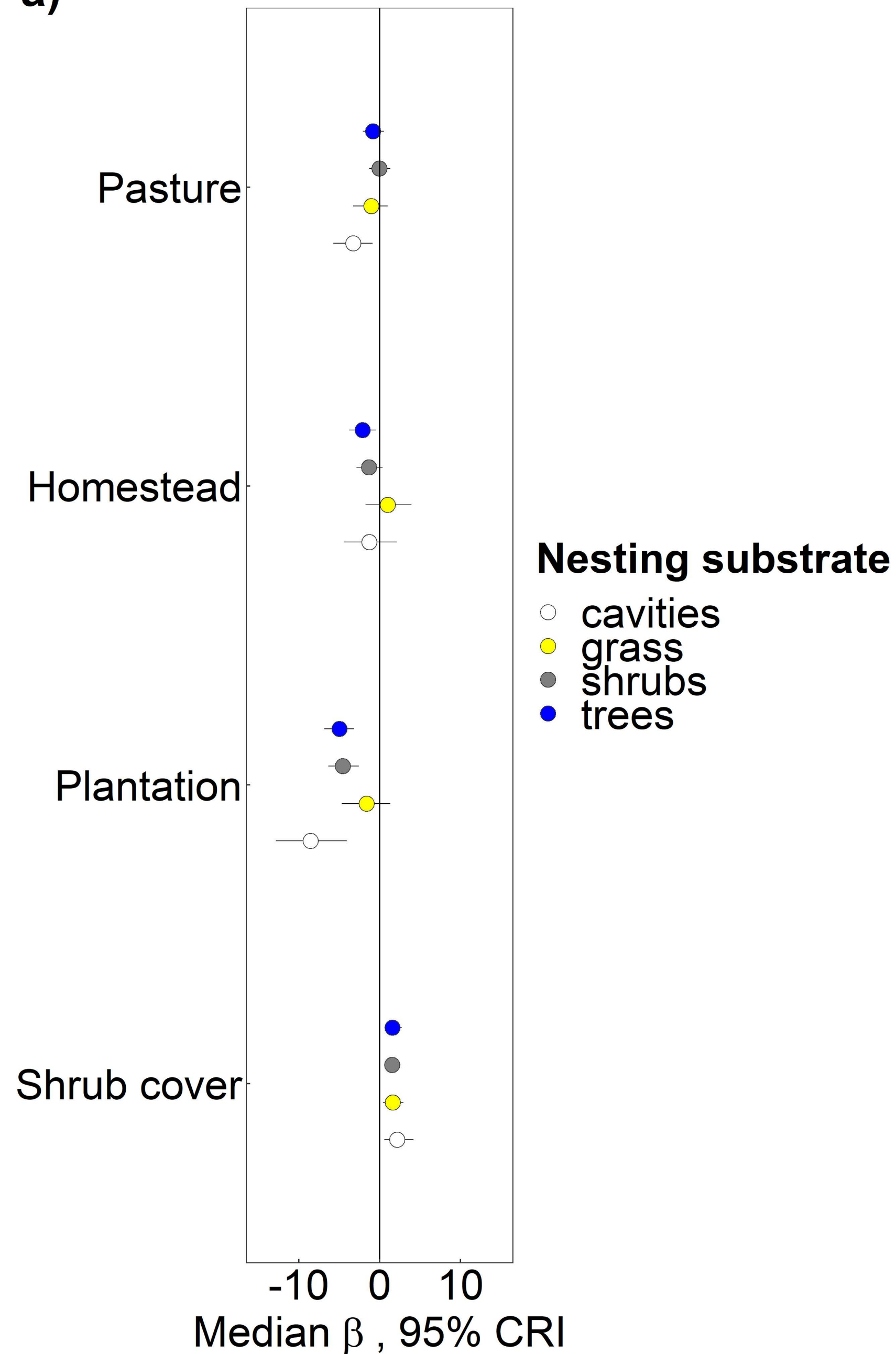
a) Nest substrate effects
