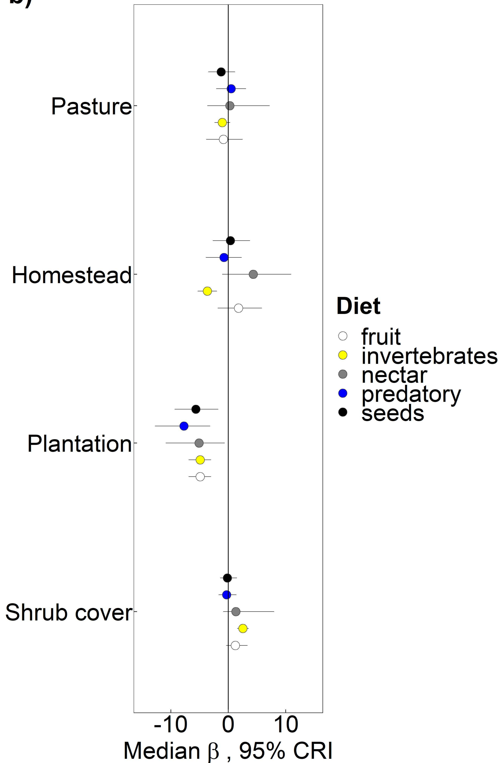
b) Diet effects
